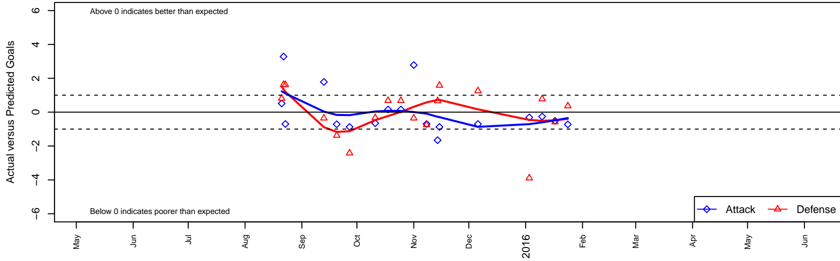
Southlake Select Lightning B98 Dots are actual minus expected GF (blue circles) and GA (red triangles). Blue line is smoothed change in attack strength. Red is smoothed change in defense strength.
